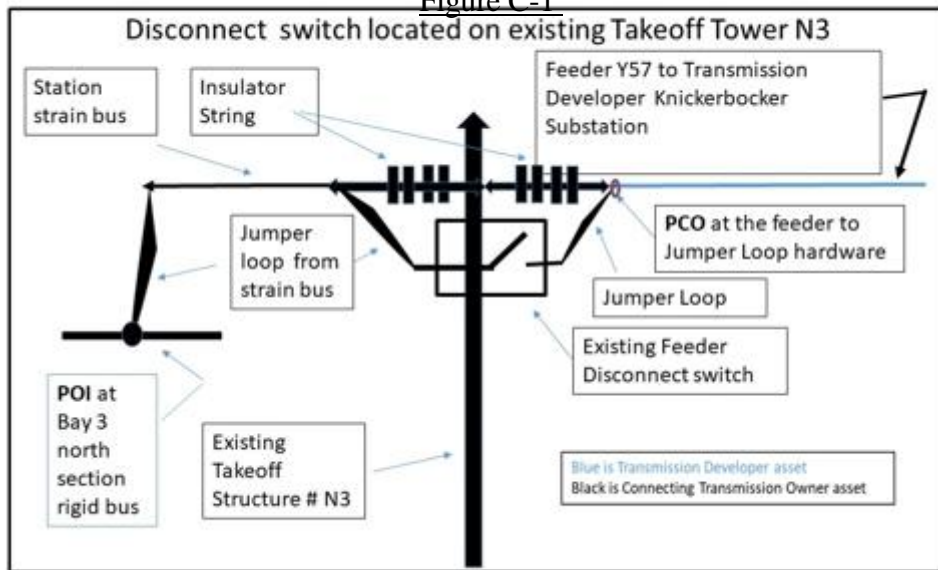
Y57 PCO/ POI one-line
