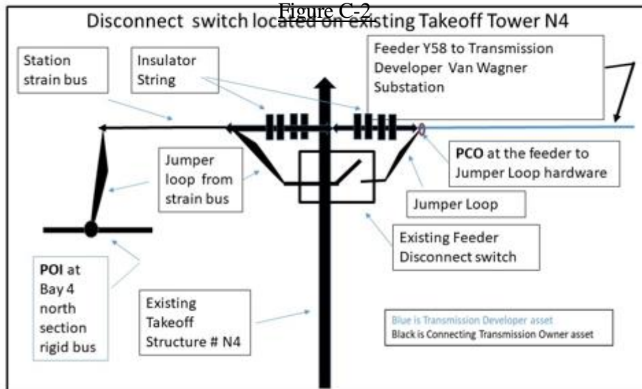
Y58 PCO/ POI one-line
