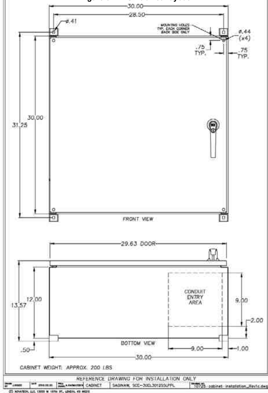
Figure 5 - RTU Cabinet Layout
