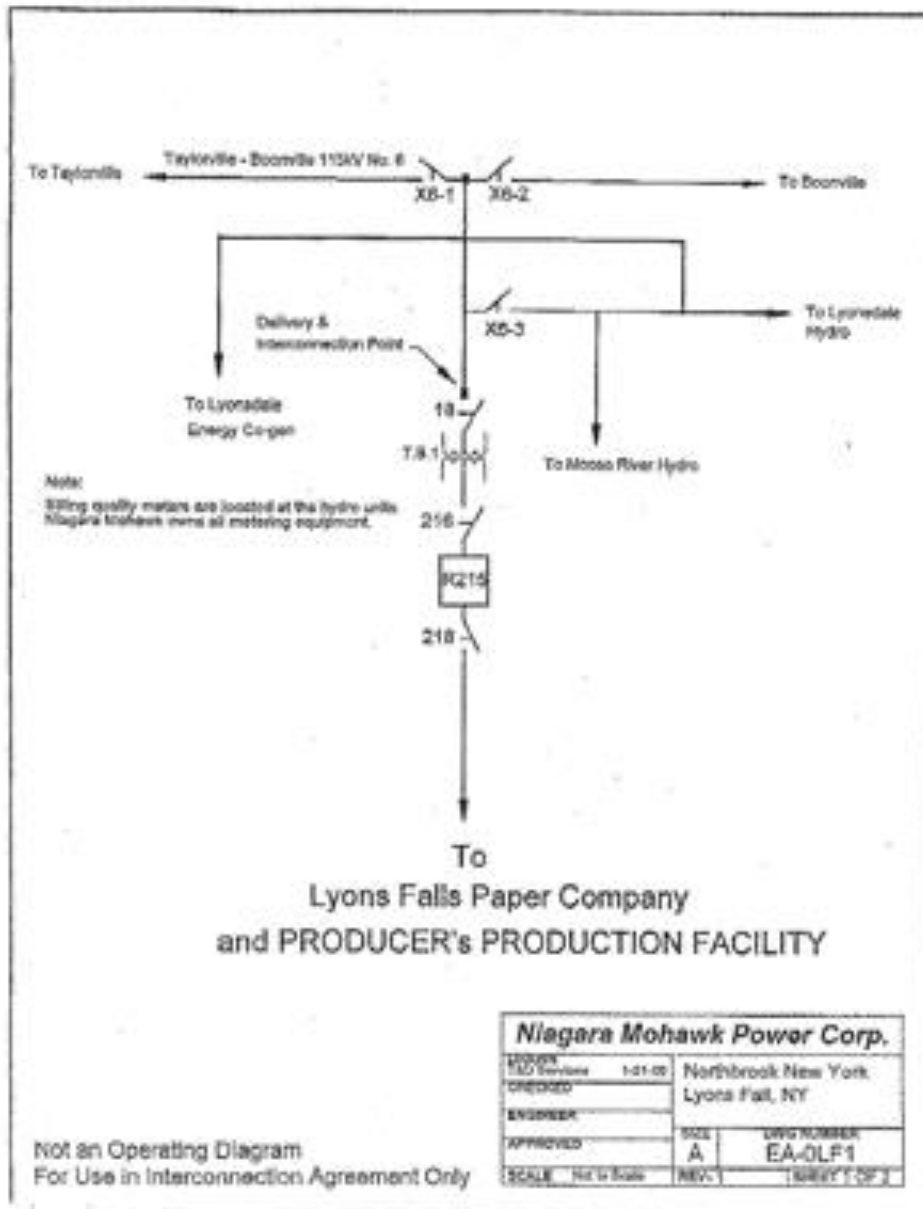
Northbrook One-Line Diagram
