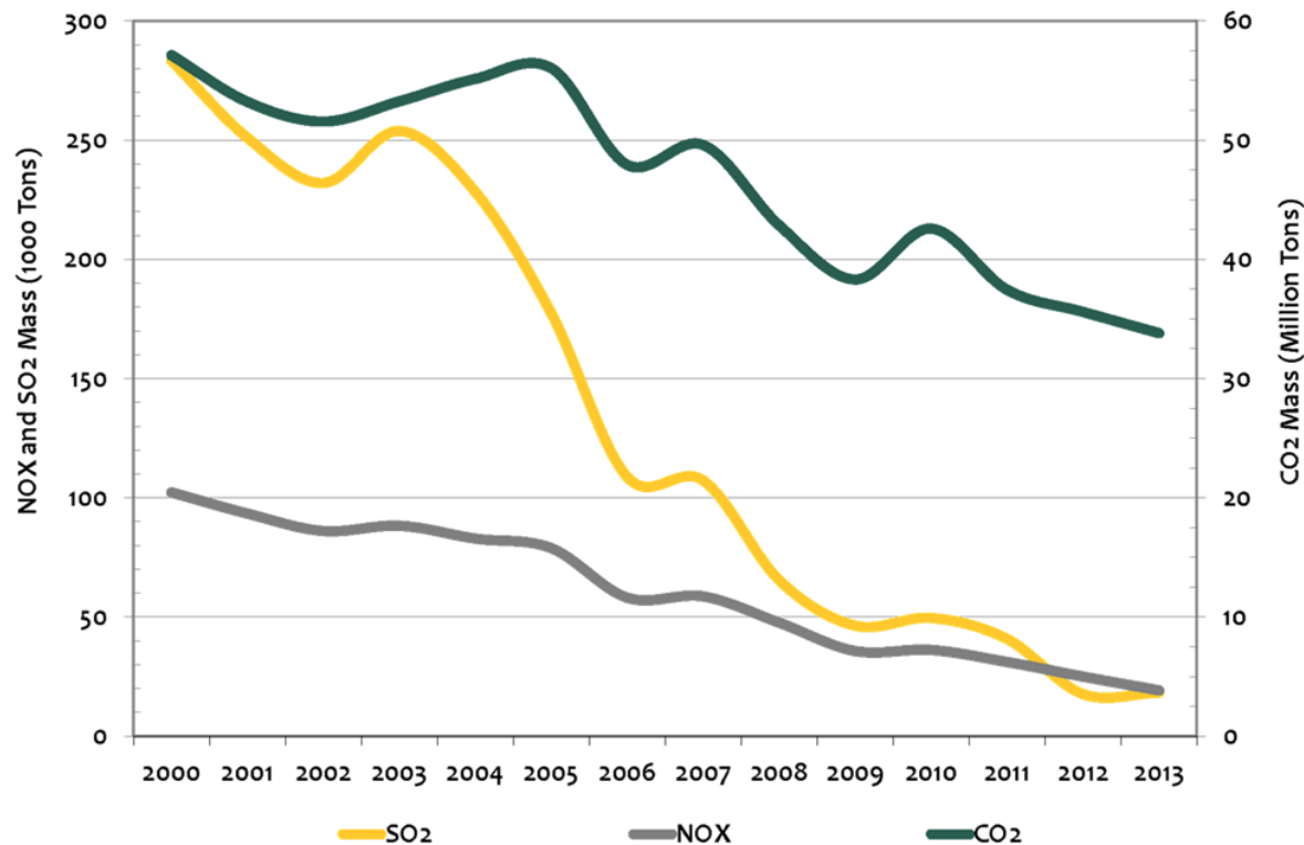
Emission Rates from Electric Generation in New York State: 2000-2013
