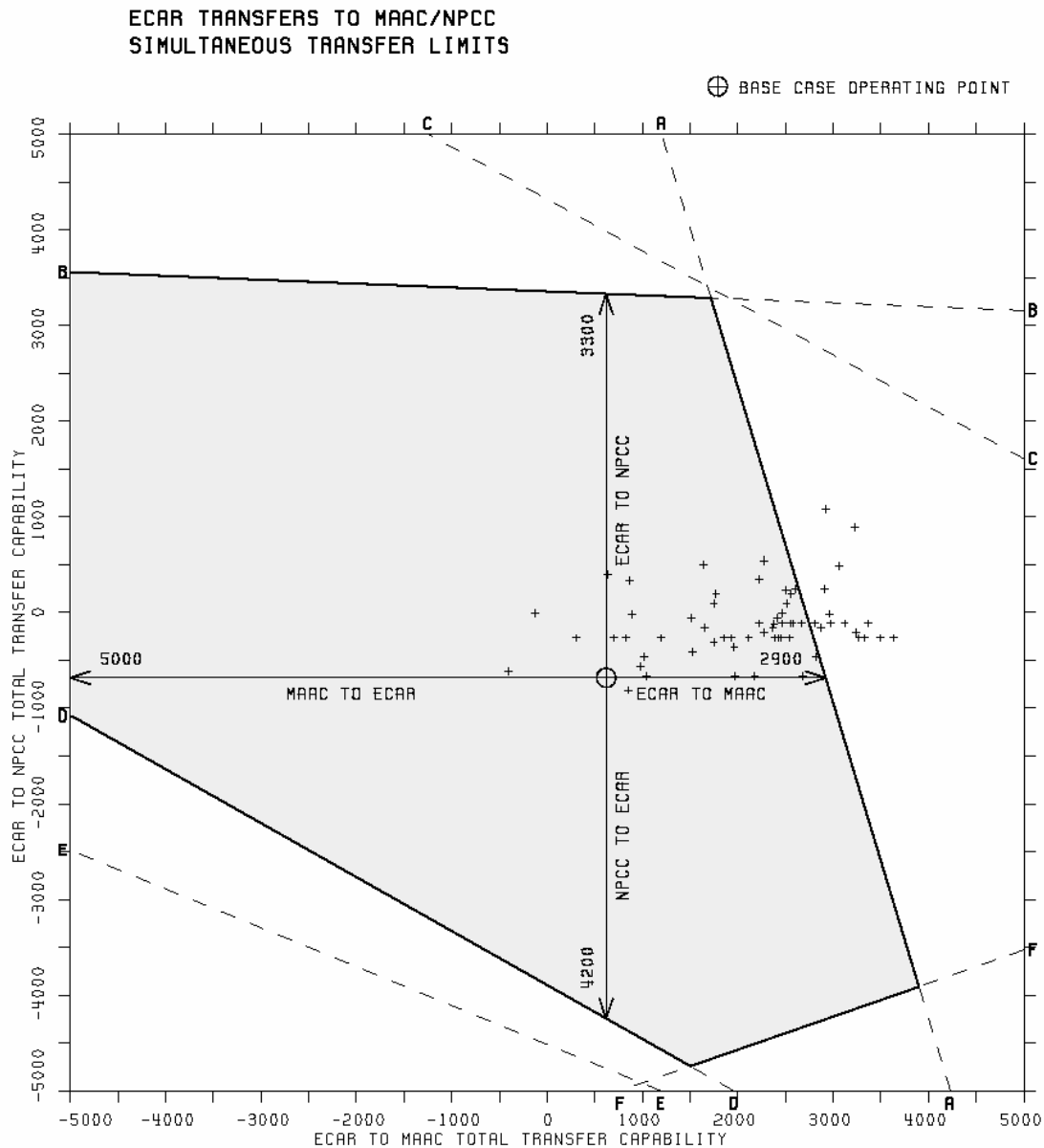
Figure 2B 2001 Summer Study Simultaneous FCTTC and Scheduled Interchange ('+') ECAR to MAAC/ NPCC
