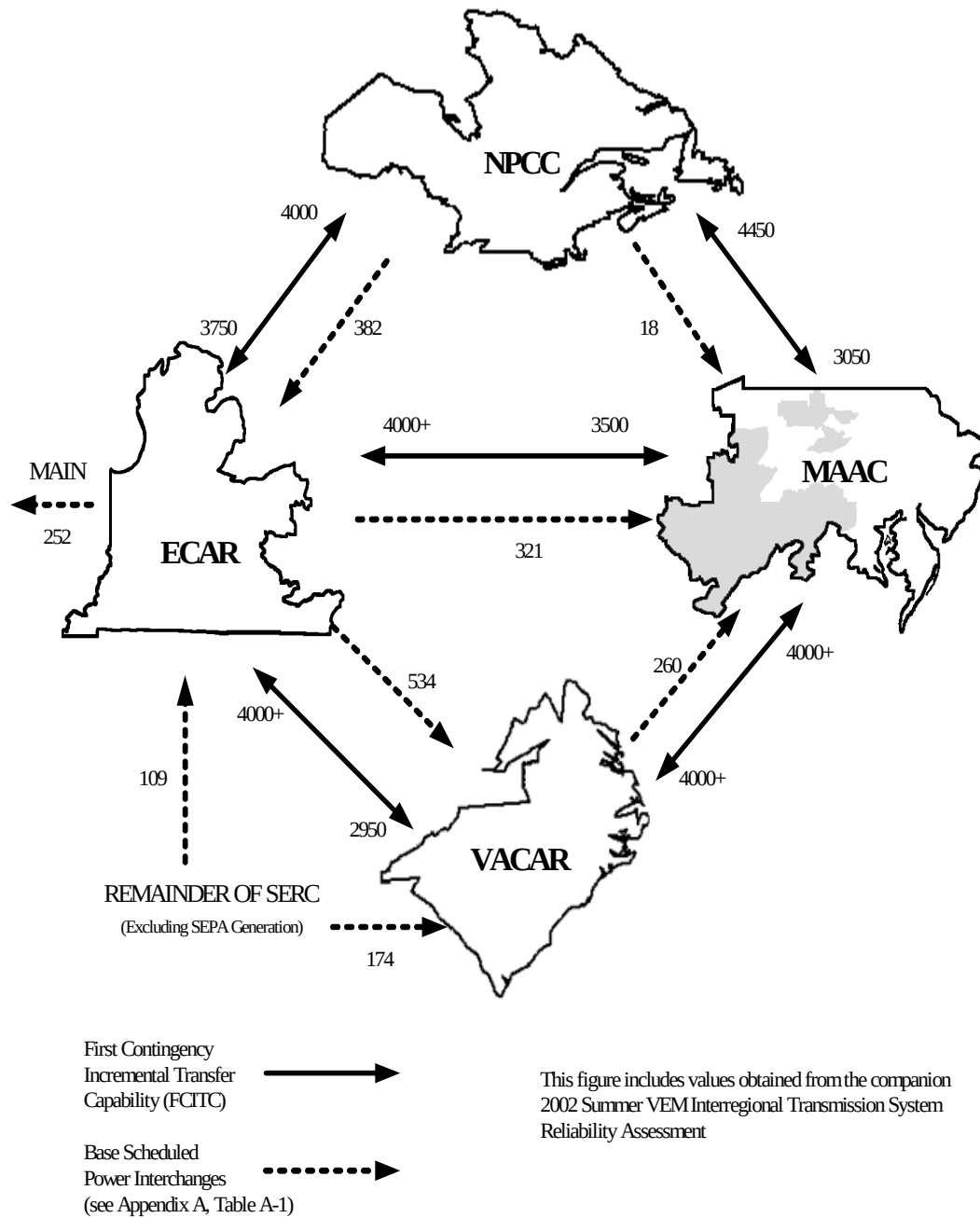
Figure 4 Non-simultaneous Interregional Transfer Capability
