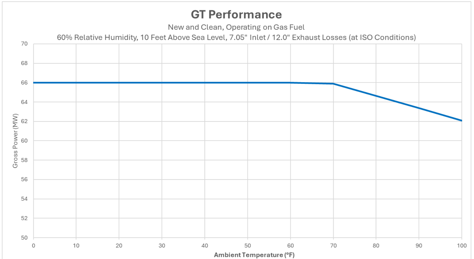
FIGURE C-1 BAYONNE ENERGY CENTER TEMPERATURE OUTPUT CURVE
