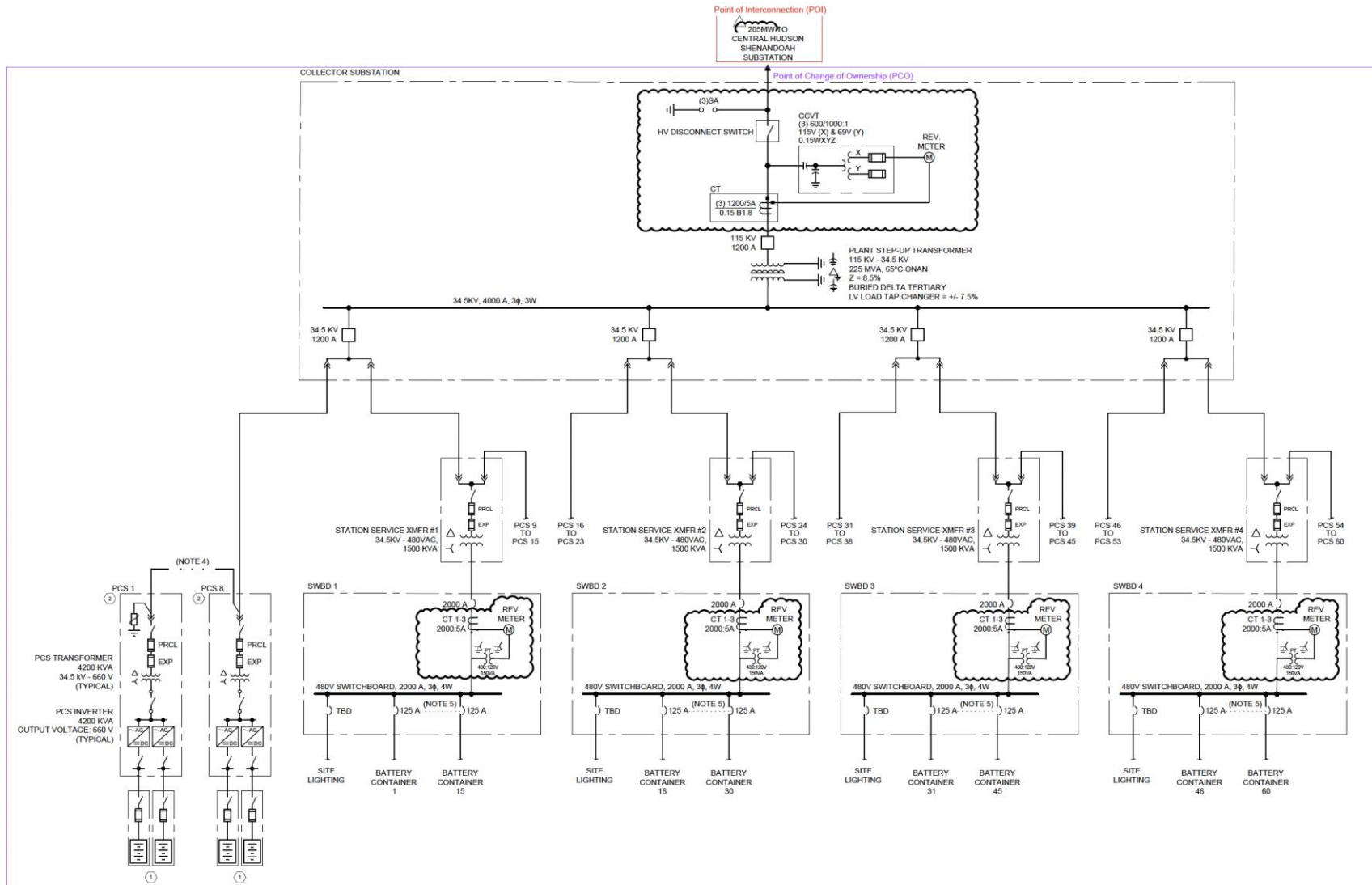
Figure A-1 Simplified One-Line Diagram
