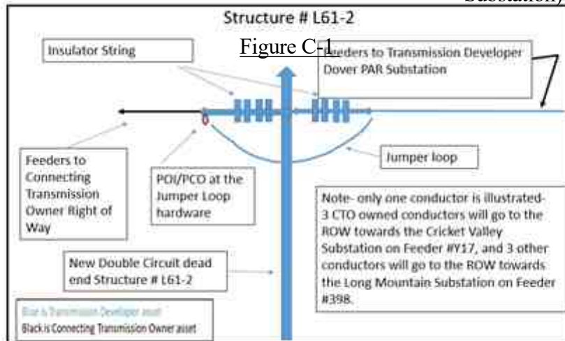
#398 & Y17 POI / PCO one-line
