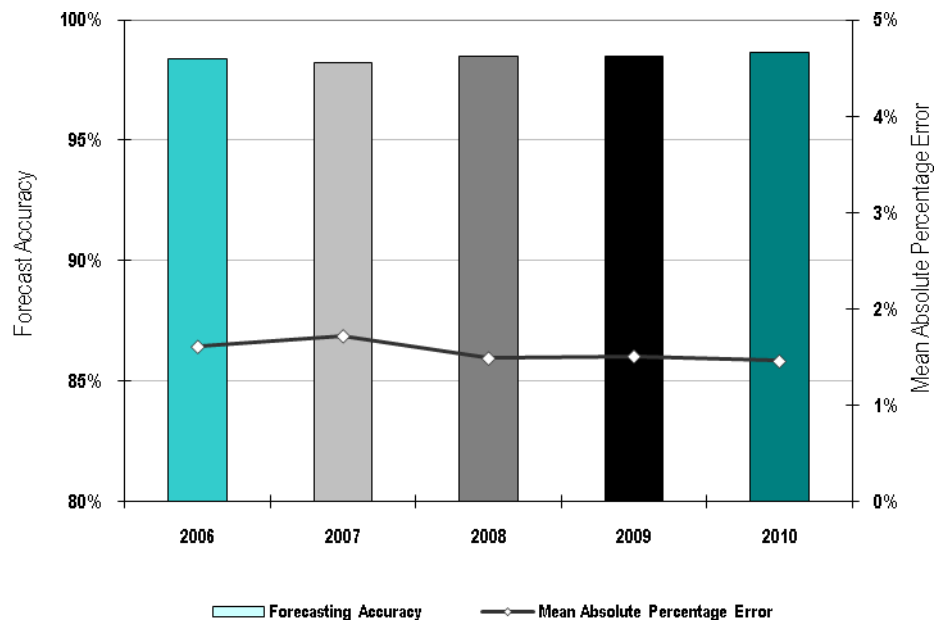
NYISO Average Load Forecasting Accuracy 2006-2010
