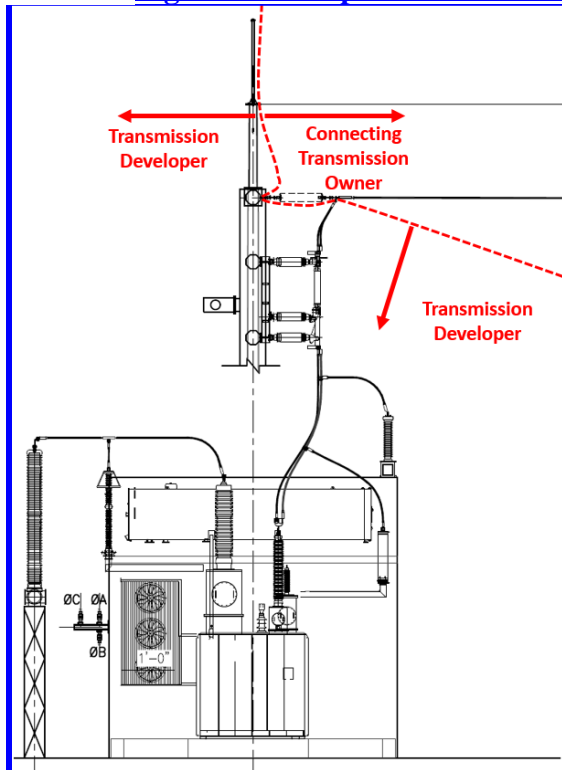
Figure C-4: Representative Connecting Transmission Owner Owned Deadend Interconnection Drawing*
