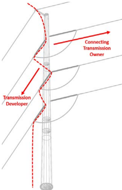
Figure C-4: Representative Connecting Transmission Owner Owned Deadend Interconnection Drawing*
