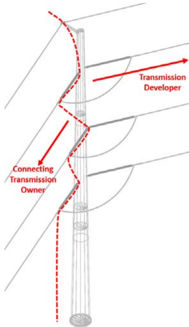
Figure C-1: Representative Transmission Developer Owned Deadend Interconnection Drawing*
