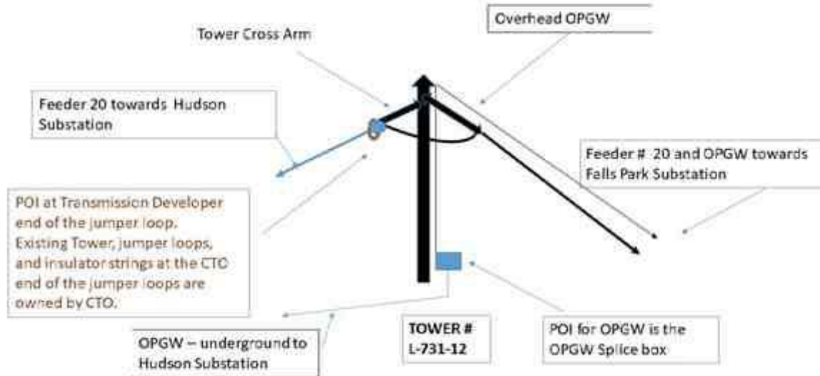
POI for #20 to Falls Figure C-3
