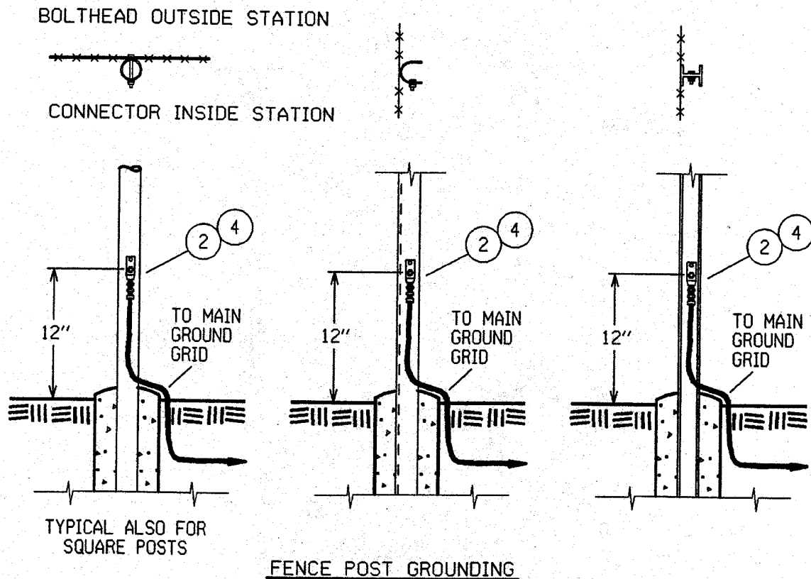
FENCE GROUNDING DETAILS FIGURE 7
