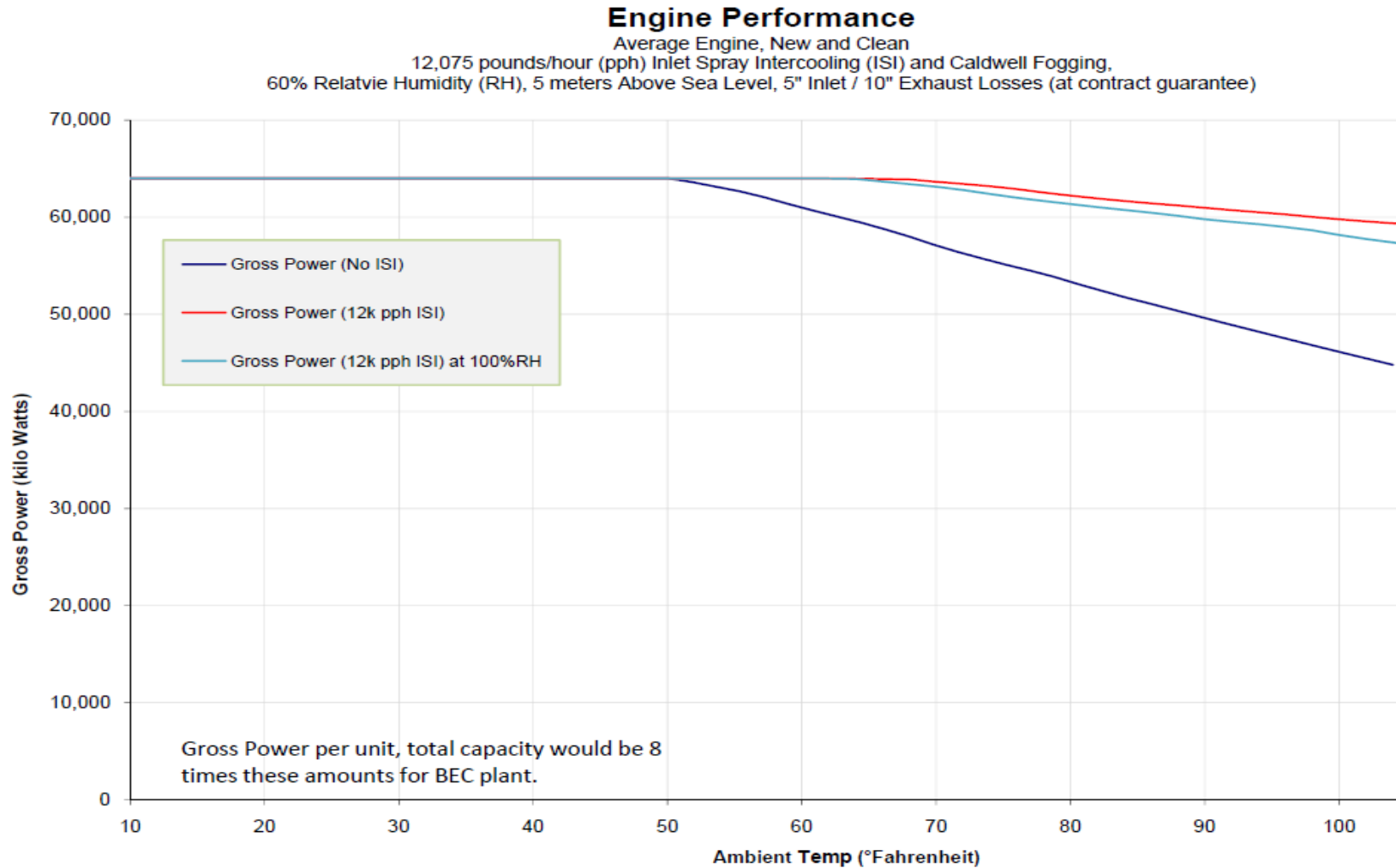
FIGURE C-1 BAYONNE ENERGY CENTER I TEMPERATURE OUTPUT CURVE
