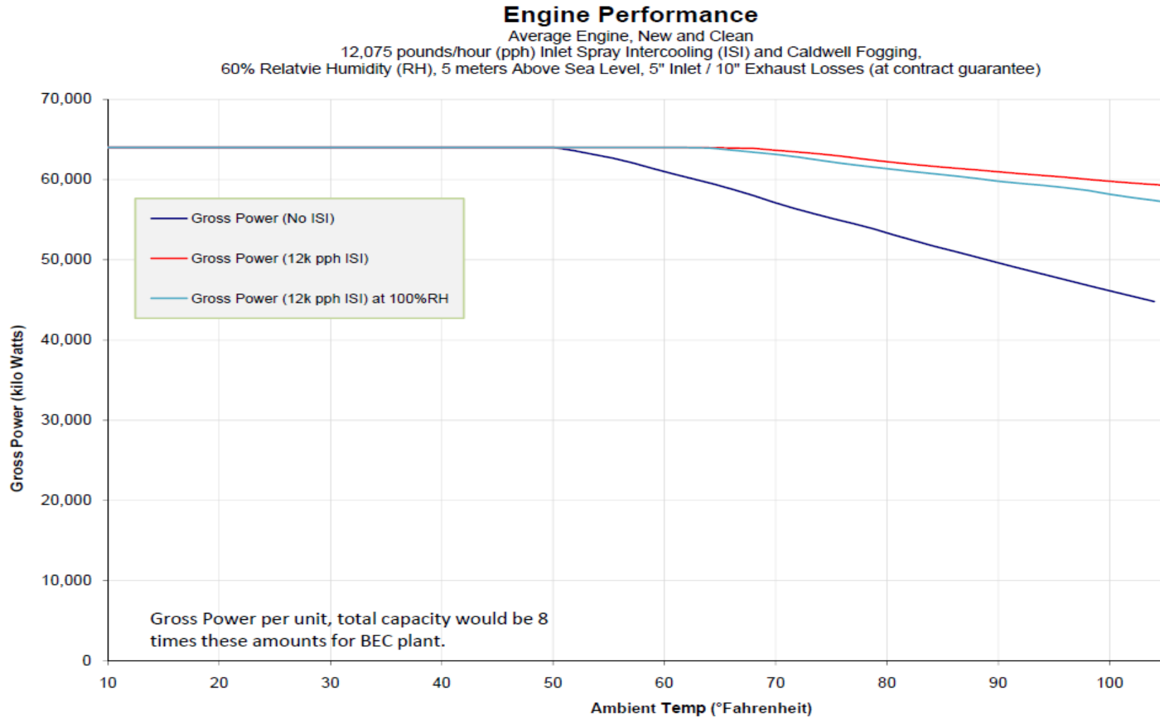
FIGURE C-1 BAYONNE ENERGY CENTER I TEMPERATURE OUTPUT CURVE
