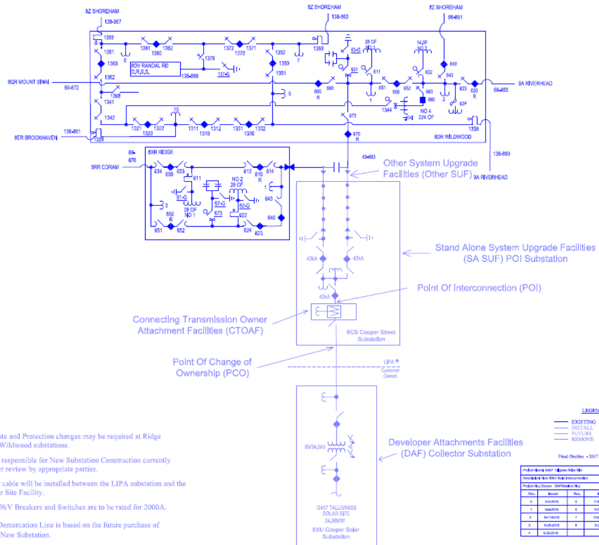
Figure A-1 System One Line
