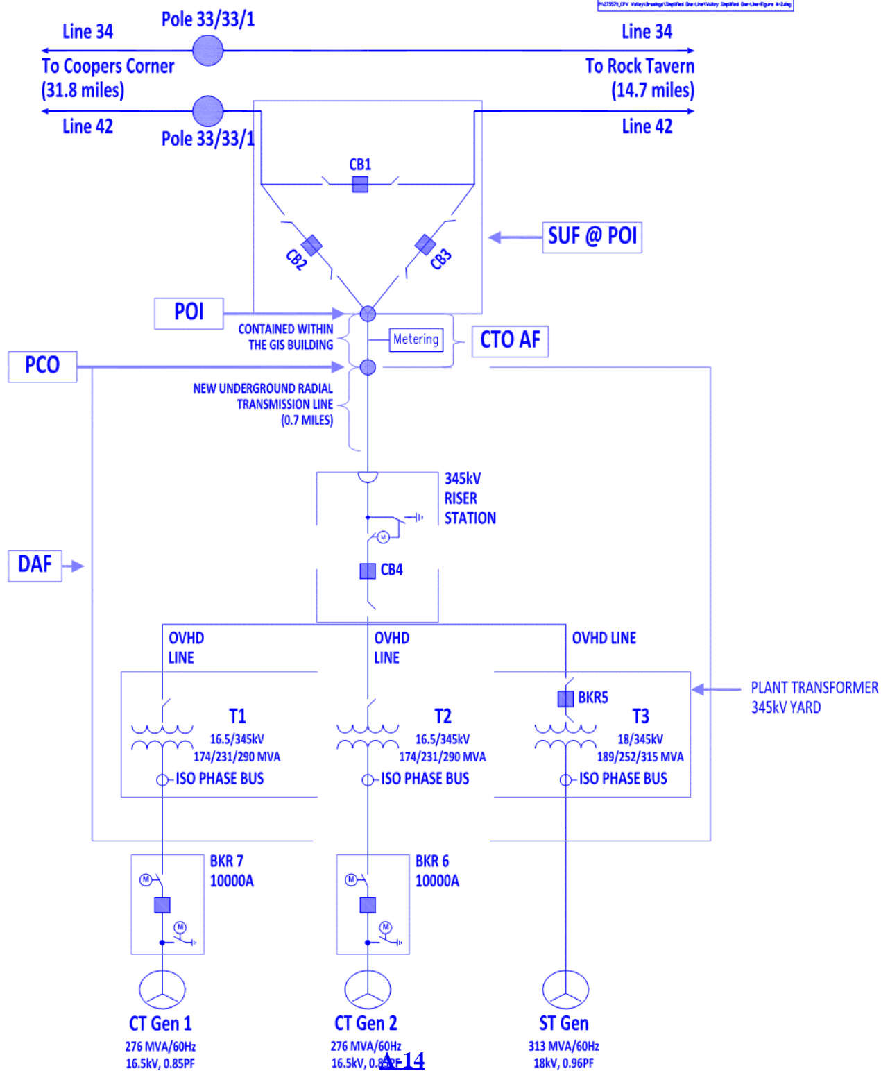
Figure A-2 CPV Valley Energy Center One-Line
