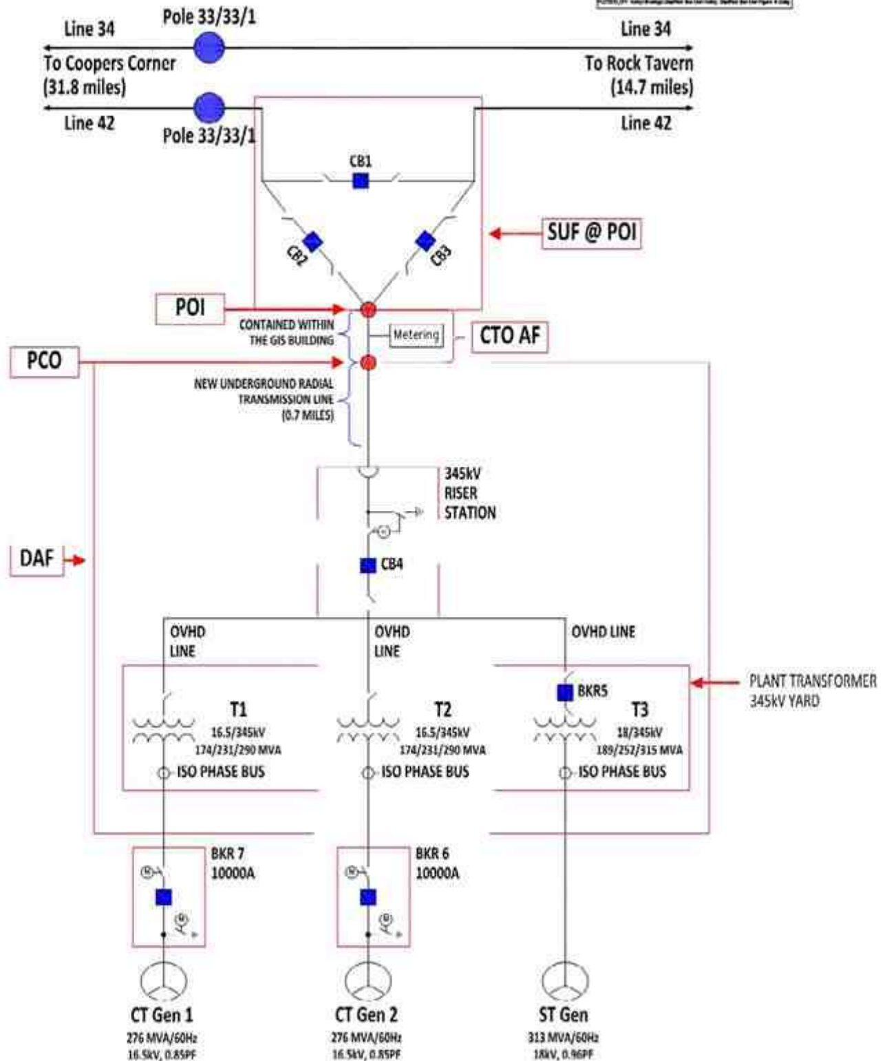
Figure A-2 CPV Valley Energy Center One-Line
