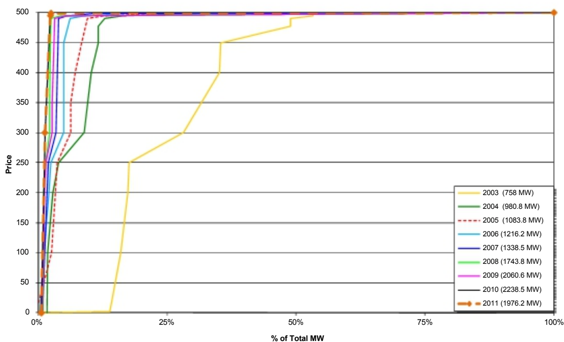
Figure 6: 2003 - 2011 ICAP/SCR Curtailment Bid Curves
