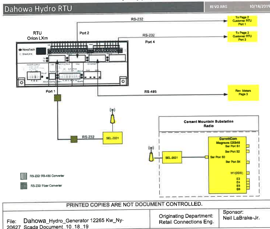
Figure 1 – RTU Functional Diagram Temporary proposal
