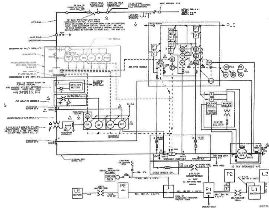
Figure 4 – Interconnection Plan
