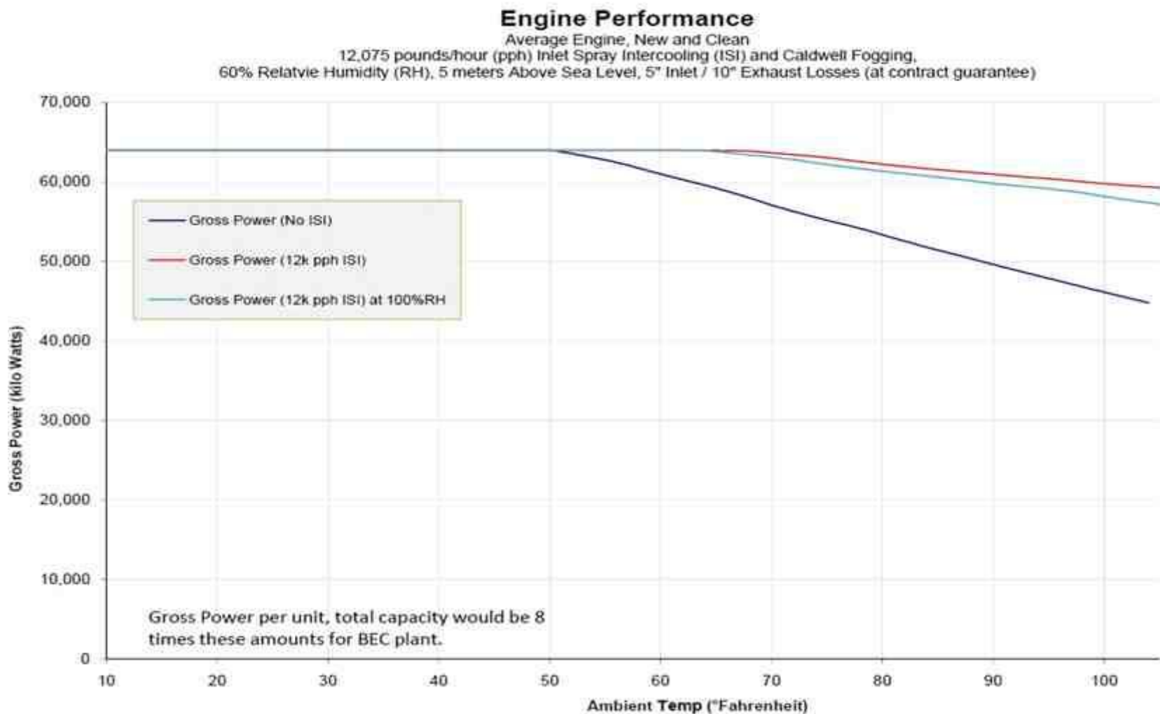
FIGURE C-1 BAYONNE ENERGY CENTER TEMPERATURE OUTPUT CURVE
