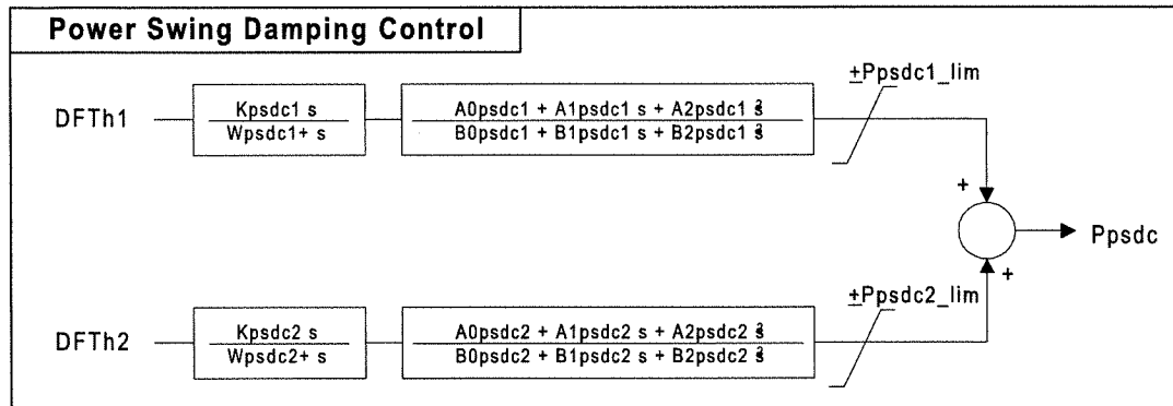
Figure 4.5.3-1 PSDC Block Diagram
