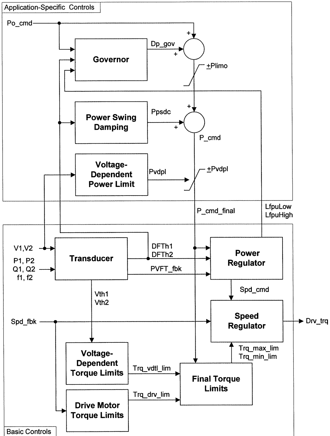
Figure I-1. Overview of VFT Controls.
