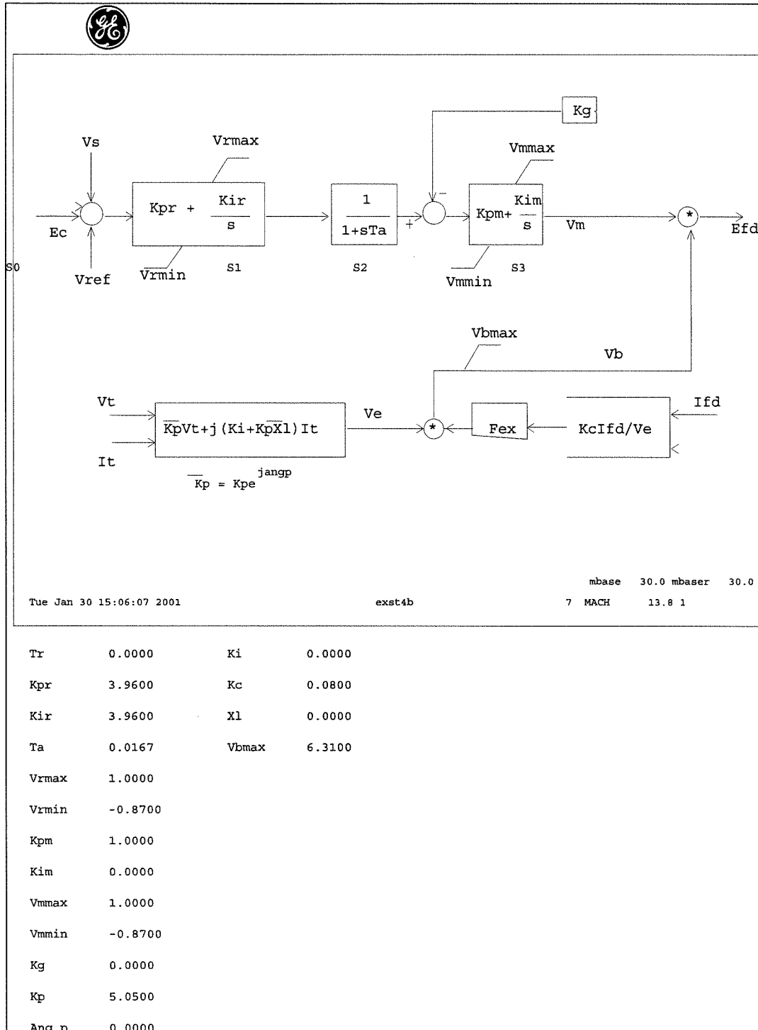
Figure A-2 Bus 7 ExciterModel
