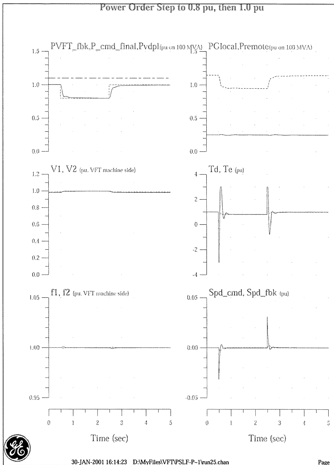
Figure 5.5-2 Small Step in Power Order
