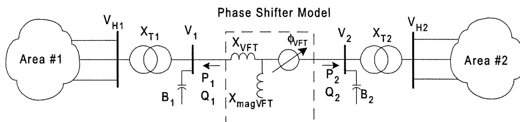
Figure 3-1. VFT Power Circuit for Loadflow Analysis
