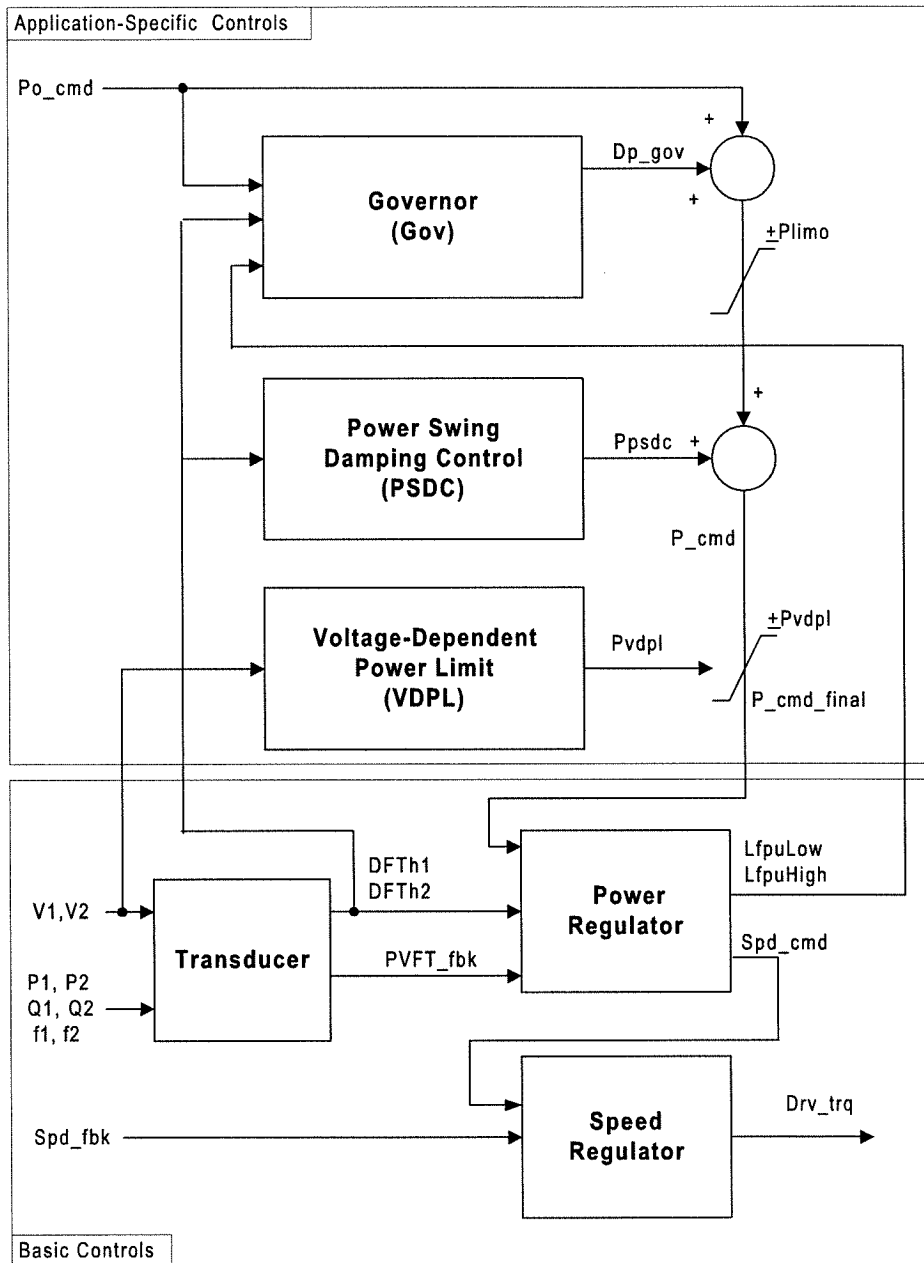
Figure 4.1-2 Overview of VFT Controls
