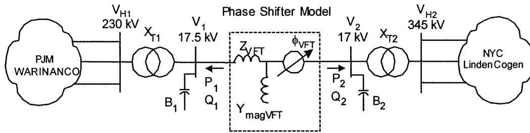
Figure 1-3. Linden VFT Model for Load flow Analysis.
