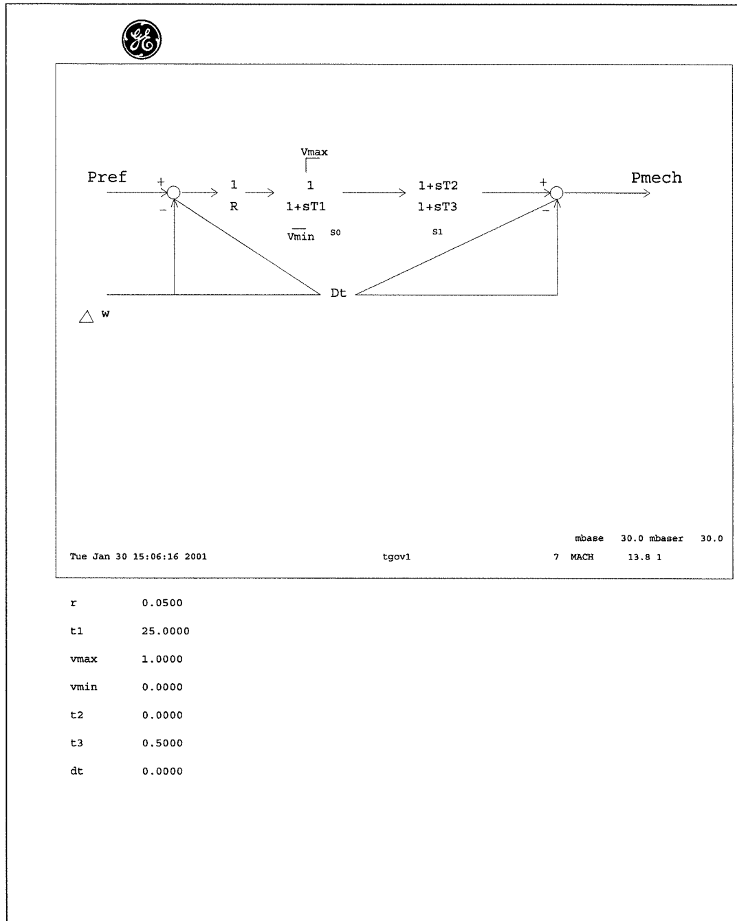
Figure A-3 Bus 7 Governor Model
