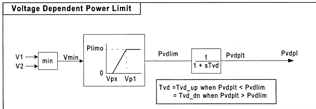
Figure 4.5.1-1 VDPL Block Diagram
