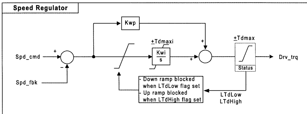
Figure 4.3-2 Speed Regulator
