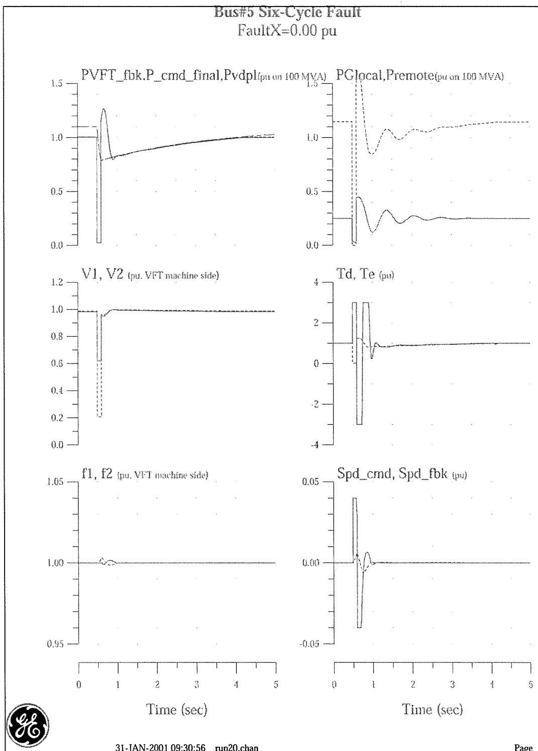
Figure 5.2-1 Six-Cycle Stub Fault
