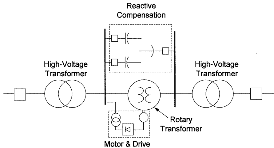
Figure 1-1. Typical Elements of a VFT Installation.
