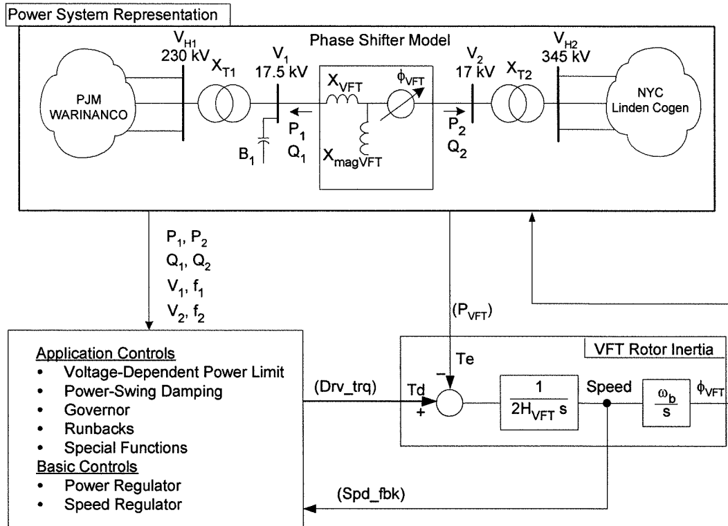
Figure 1-5. Overview of VFT Dynamics Model.
