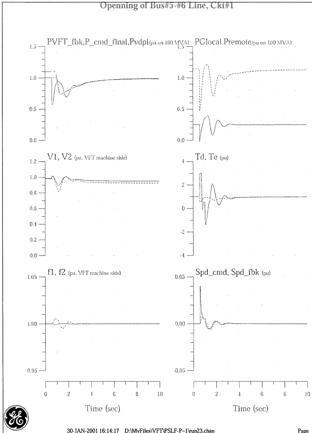
Figure 5.3-2 Line Opening Resulting in Weak Receiving System
