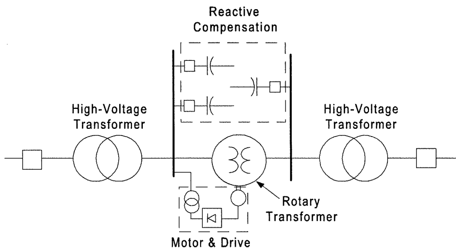
Figure 2-1 Typical Elements of a VFT Installation
