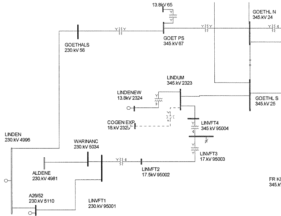
Figure 1-4. Linden VFT Short Circuit Model.
