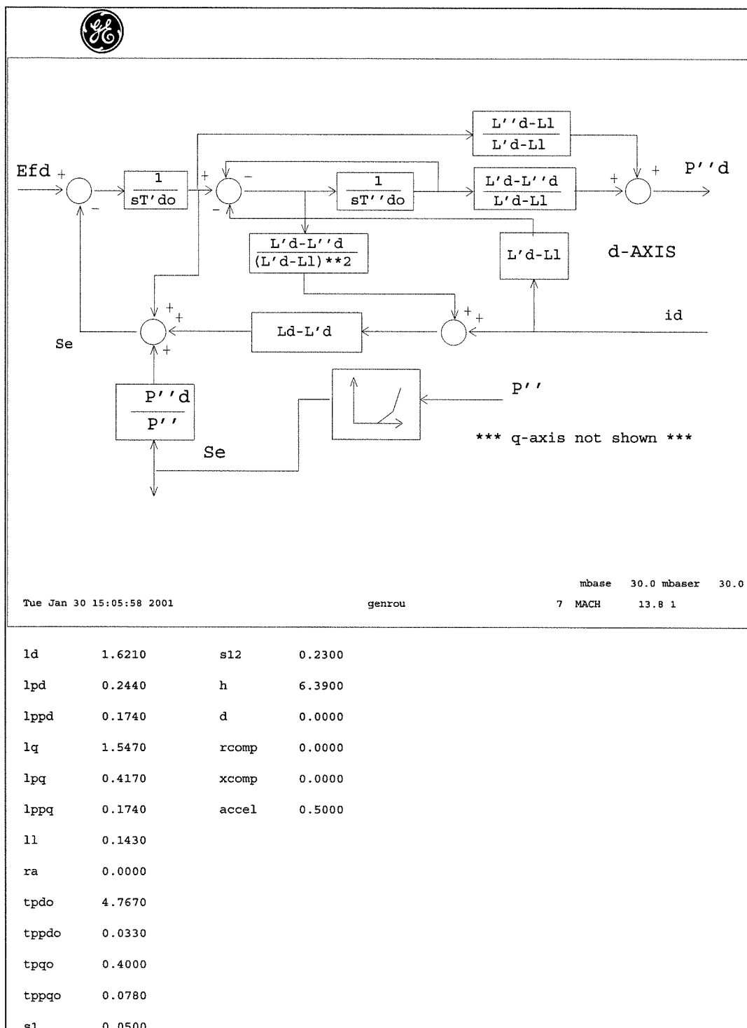
Figure A-1 Bus 7 Generator Model
