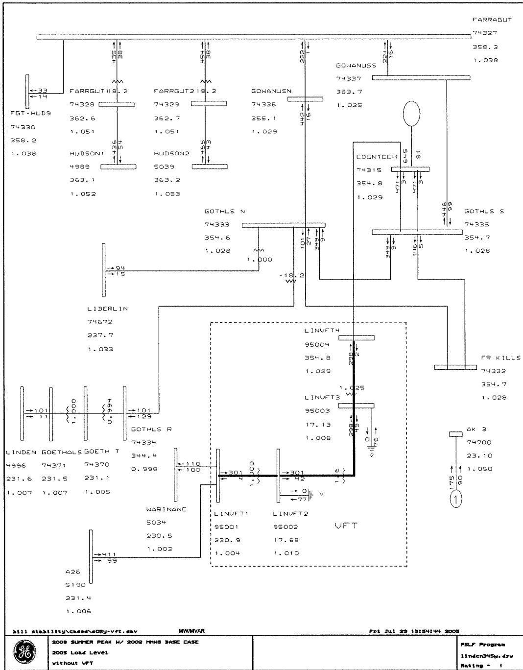
Figure 1-2. Linden VFT Connection to the Network
