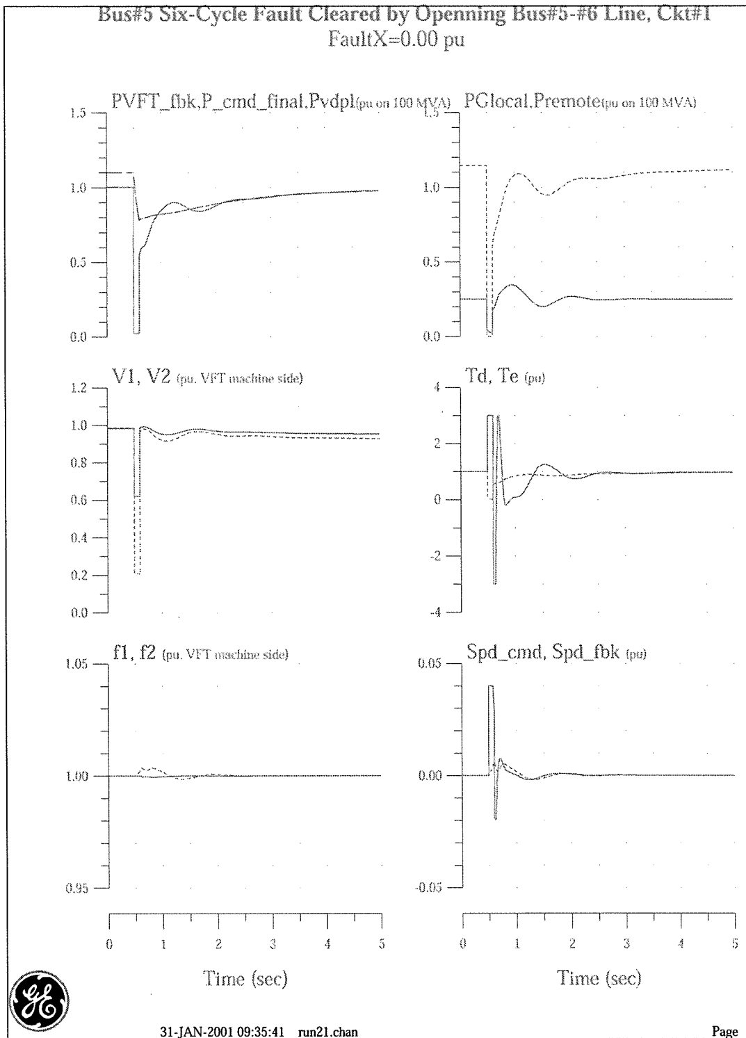
Figure 5.3-1 Six-Cycle Fault with Clearing Resulting in Weak Receiving System
