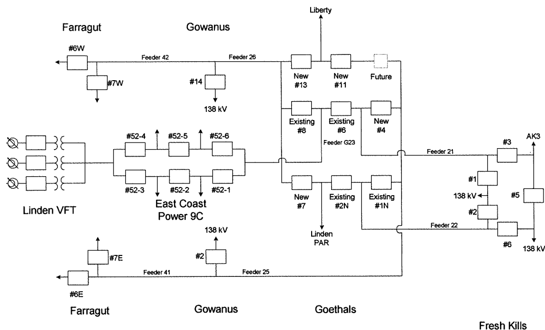
Figure 3-1. Goethals Substation Reconfiguration and Vicinity.
