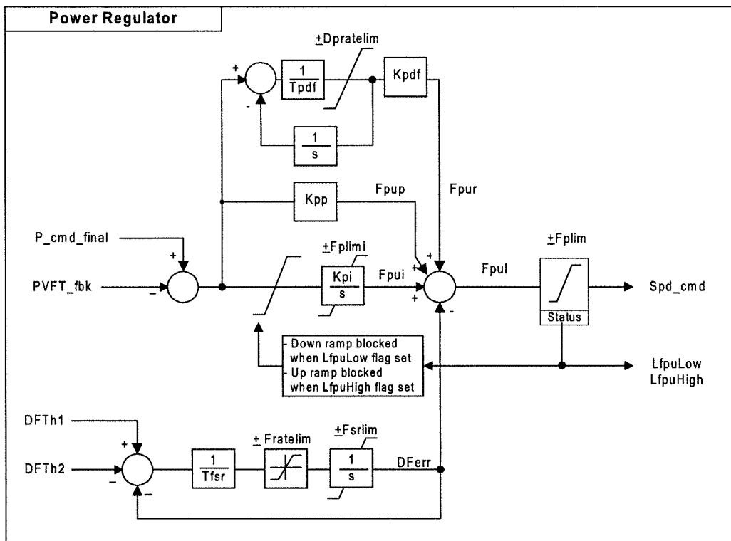
Figure 4.3-1 Power Regulator
