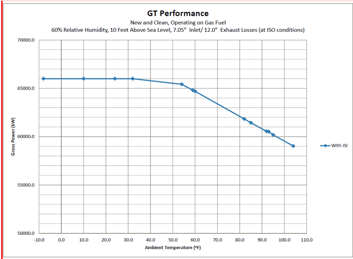
FIGURE C-2 BAYONNE ENERGY CENTER II TEMPERATURE OUTPUT CURVE
