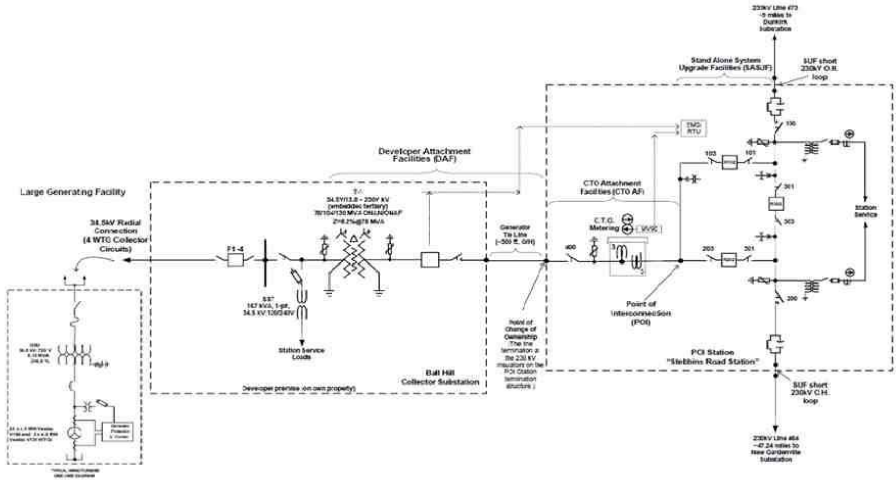
Q505 Ball Hill Wind Project Simplified One Line Schematic Figure A-1
