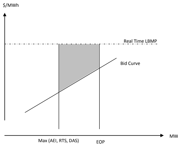
Figure 2.0(b) - Incremental Bid Curve Used to Calculate LOC
