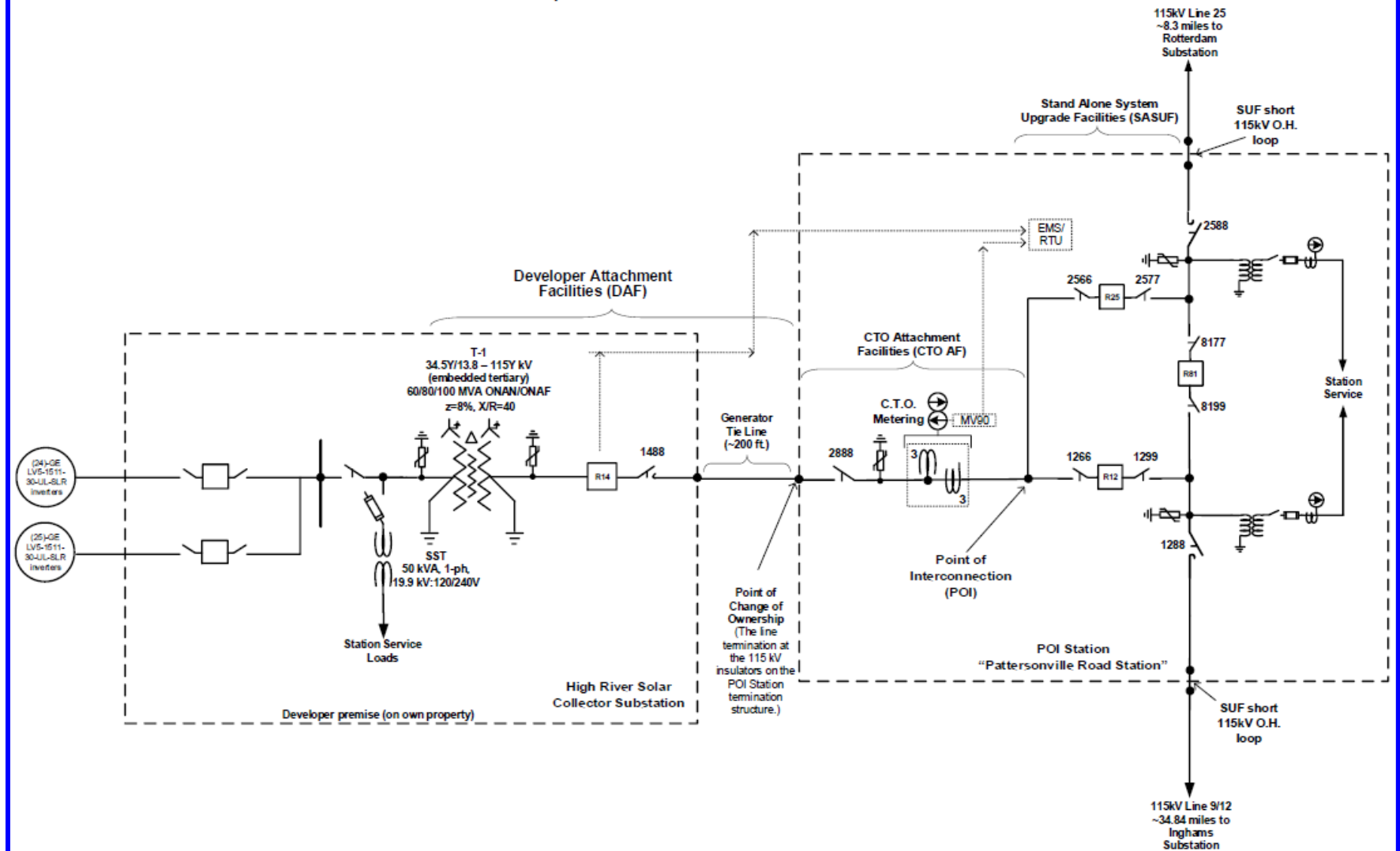
Simplified One Line Schematic
