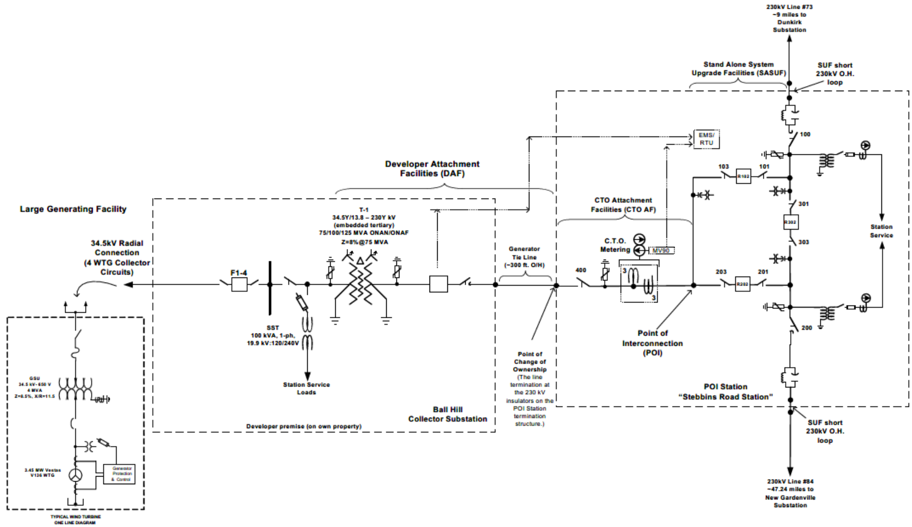
Figure A-1 Q505 Ball Hill Wind Project Simplified One Line Schematic
