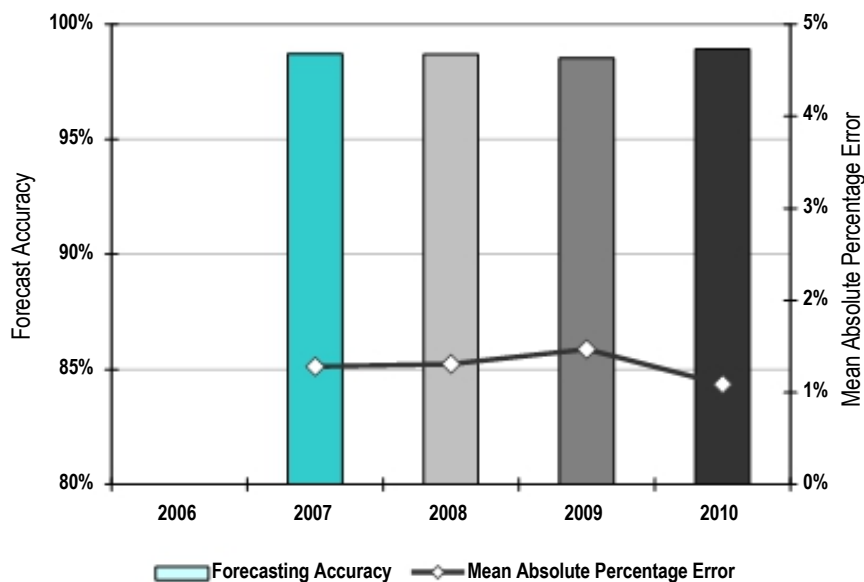
MISO Valley Load Forecasting Accuracy 2007-2010
