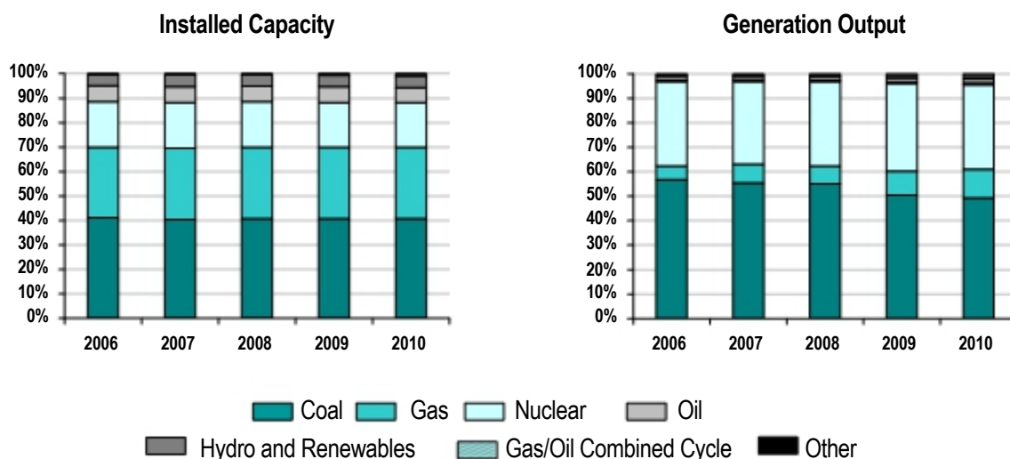
PJM Fuel Diversity 2006-2010
