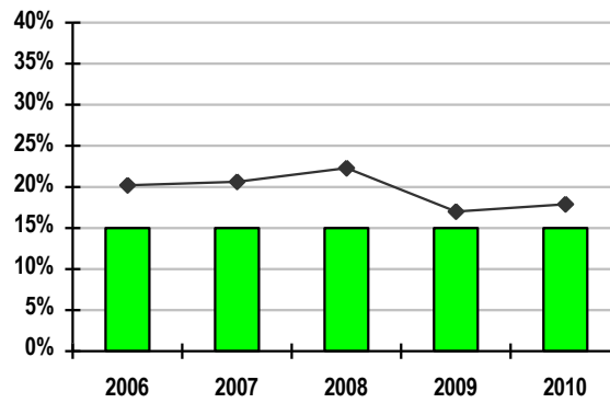
California ISO Planned Reserve Margin 2006-2010
