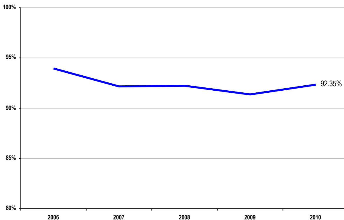
MISO Annual Generator Availability 2006 - 2010
