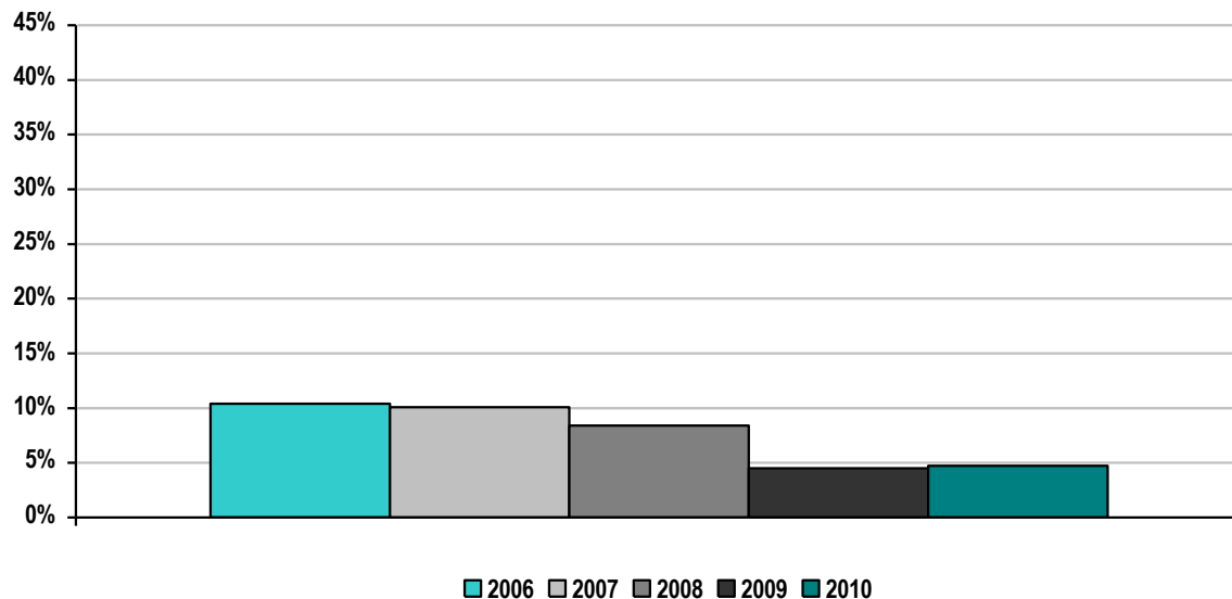
PJM Absolute Value of Unscheduled Flows as a Percentage of Total Flows 2006-2010
