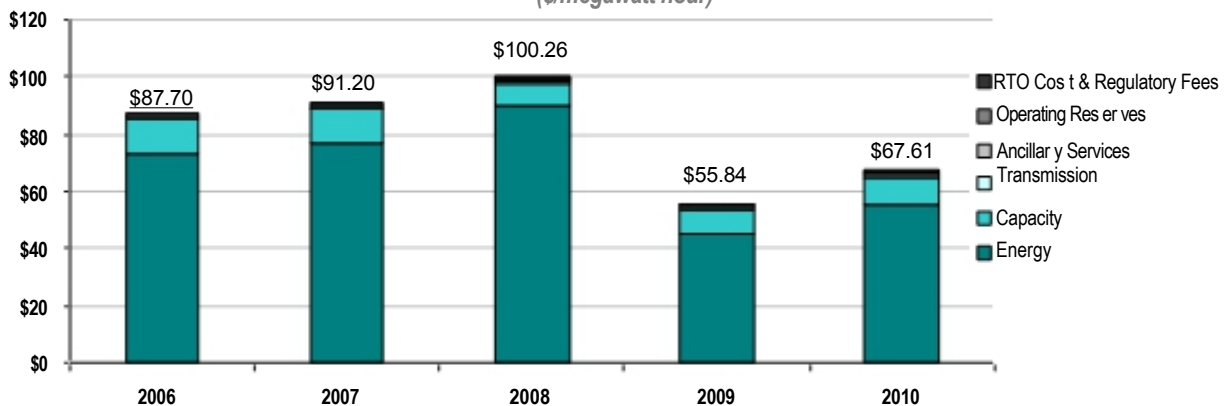
NYISO Wholesale Power Cost Breakdown ($/megawatt hour)
